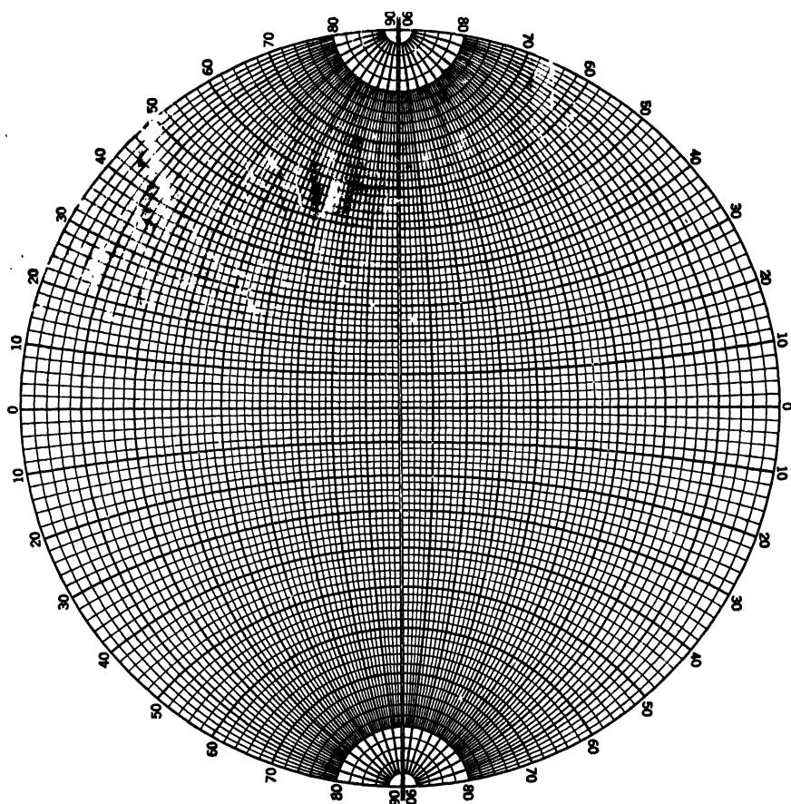
FIG. 17.—Stereographic net.
